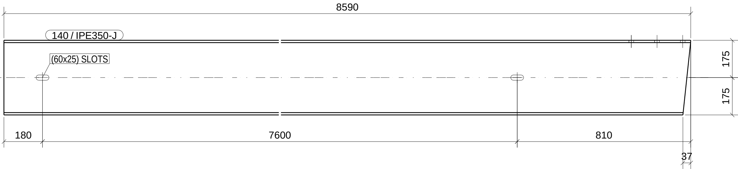
FRONT VIEW
